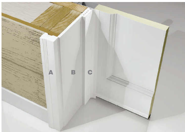
A Brick Mould B Jamb (non load-bearing) C Garage Door Stop
